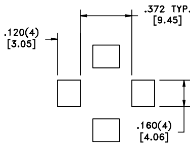
MOUNTING PATTERN
